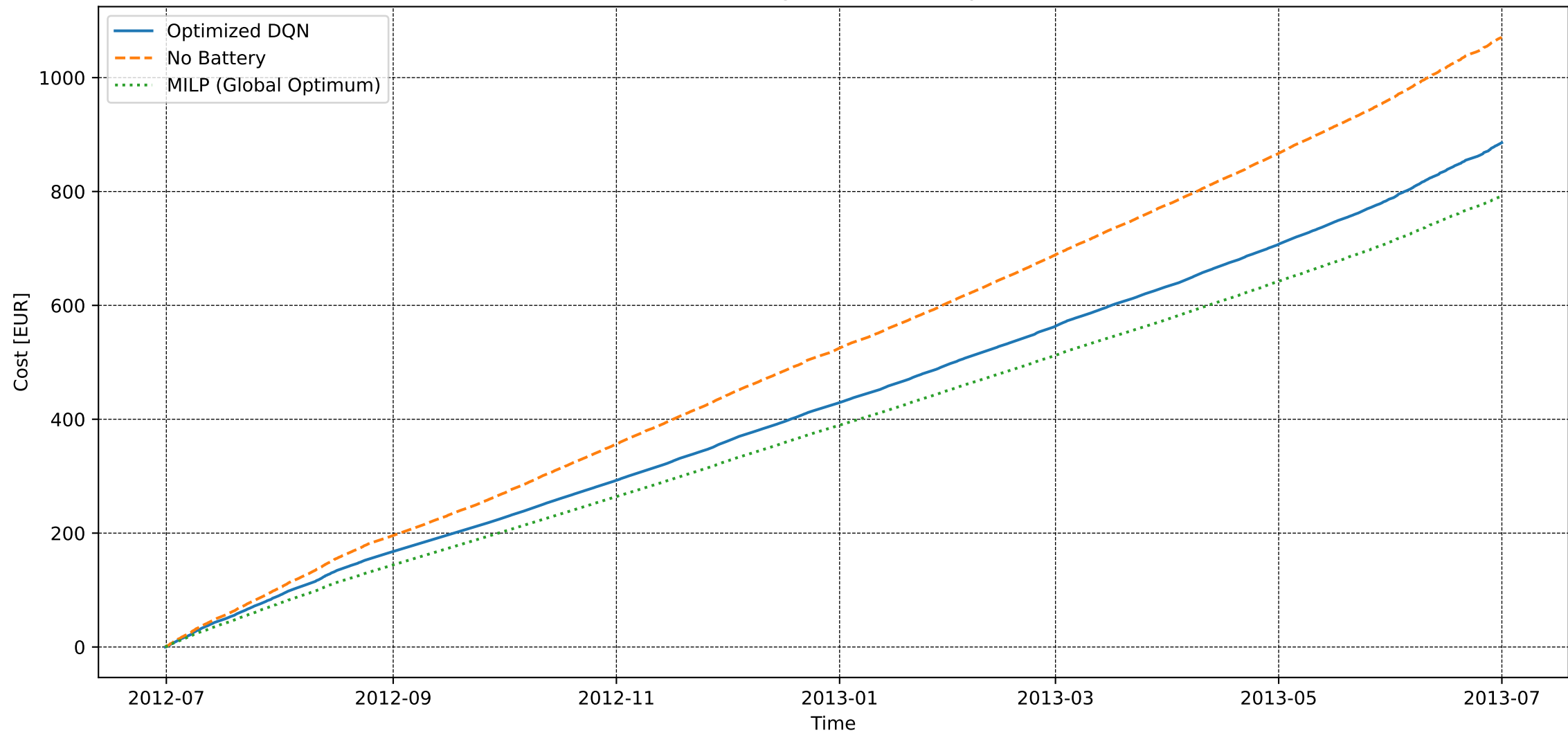
User 142 - Extended Convergence - Electricity Cost [DQN vs MILP]
